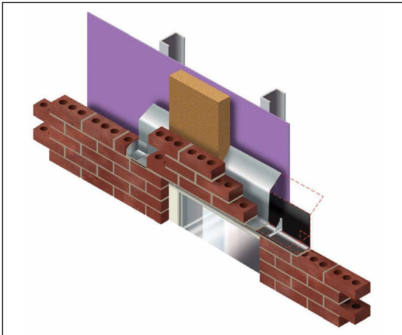
Figure 11 Lintel detail
