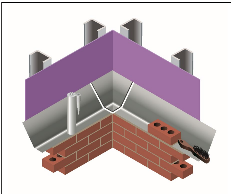
Figure 9 Trays' exposed edges sealed with METZ Sealant
